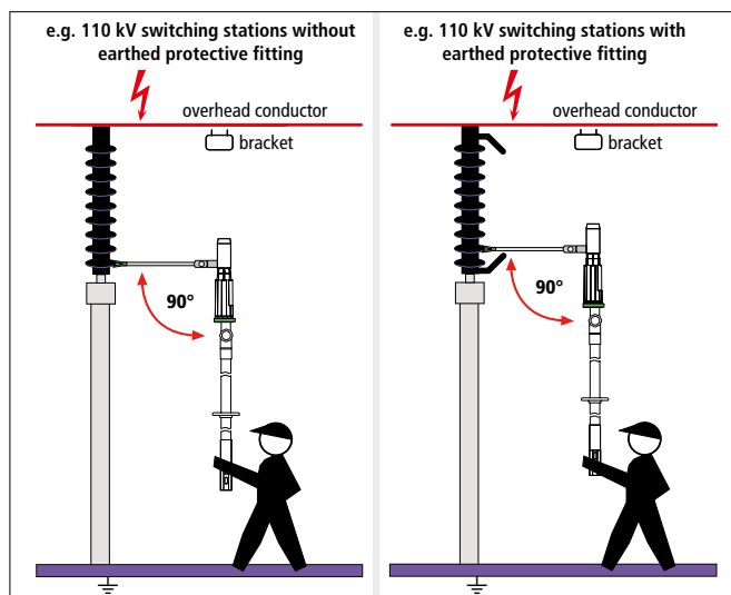
Use of an ASP distance voltage detector in an outdoor switching station.
