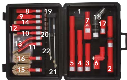
FRS ZK MS Damp Cleaning Kit Fully equipped GRP case.
