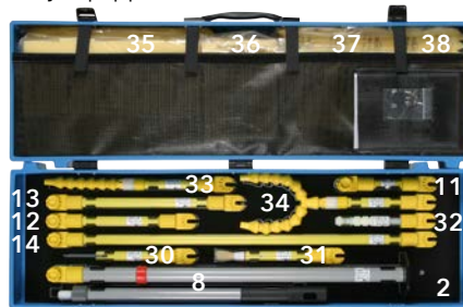
FRS ZK MS Damp Cleaning Kit Fully equipped GRP case.
